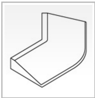
Outside 45 Degree Corner Reducer 16" x 8" x 2.25"
