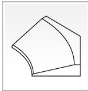
Inside 45 Degree Corner Reducer 12" x 8" x 2.25"
